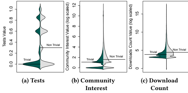
Figure 3: Distribution of Tests, Community Interest and Download Count Metrics.
