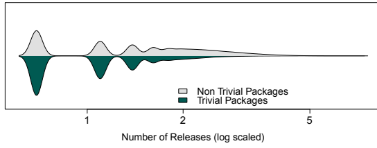
Figure 4: Number of Releases for Trivial Packages Compared to Non-trivial Packages.
