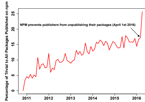
Figure 2: Percentage of Published Trivial Packages on npm .
