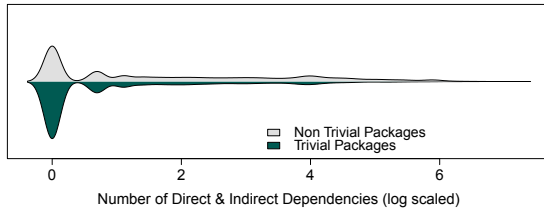
Figure 5: Distribution of Direct & Indirect Dependencies for Trivial and Non-trivial Packages ( p -value < 2.2e-16 & Cliff's Delta ( d ) -0.279 (small)).
